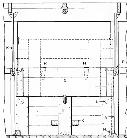
Fig. 1888. Interior Elevation of Double Grain Door.
